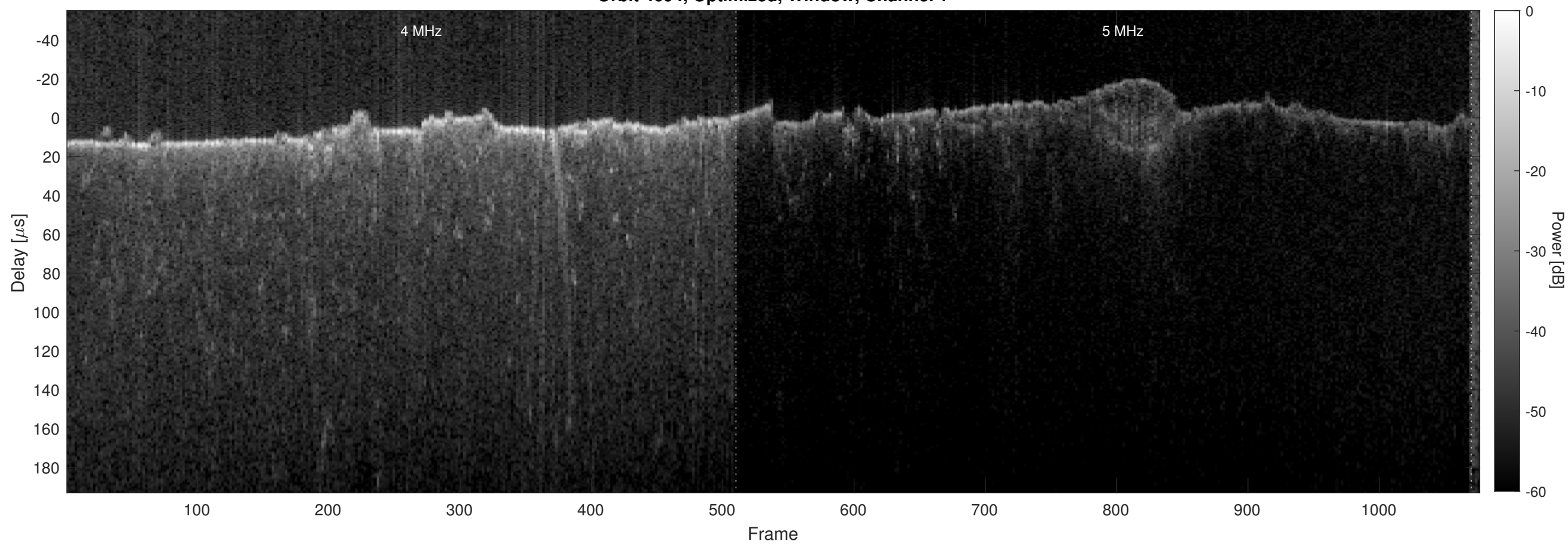
Orbit 4694, Optimized, Window, Channel 2
