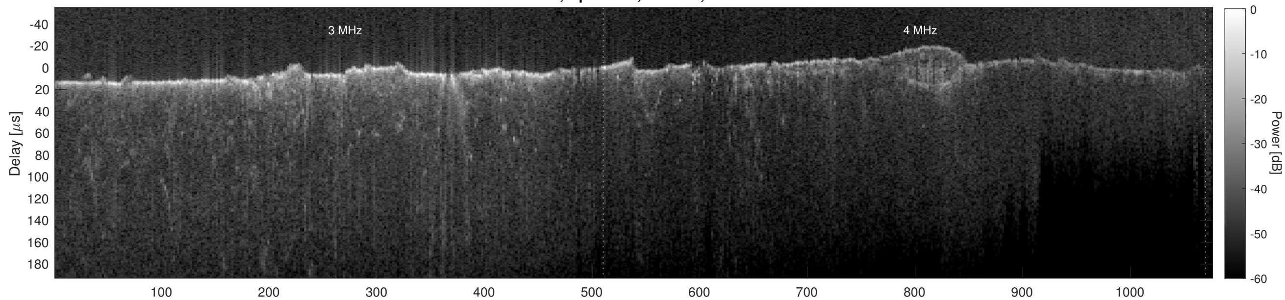
Orbit 4694, Cluttergram
