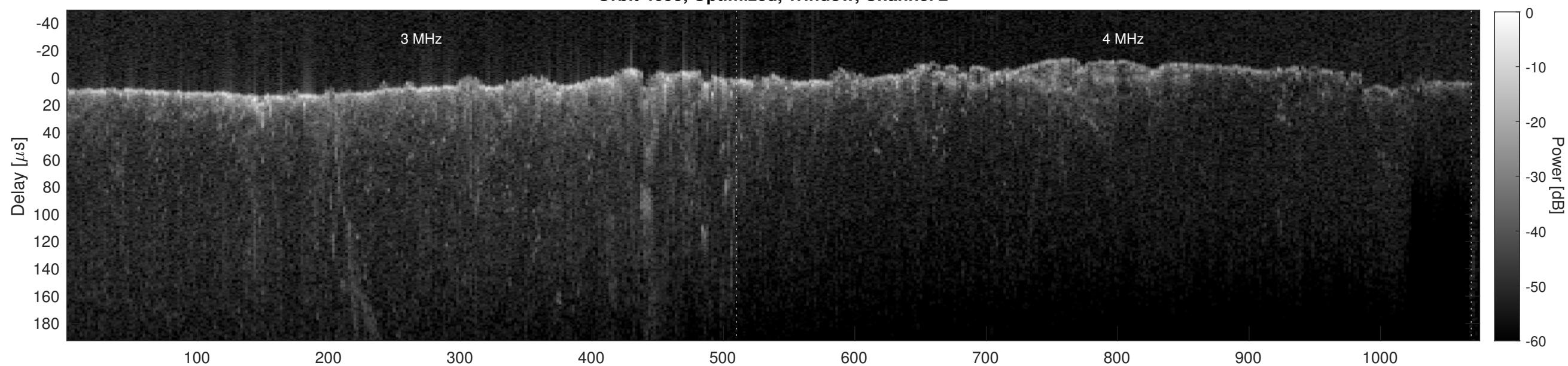
Orbit 4695, Cluttergram
