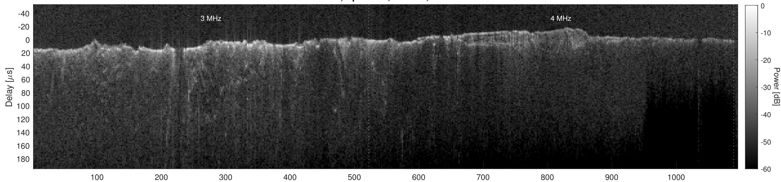
Orbit 4698, Cluttergram
