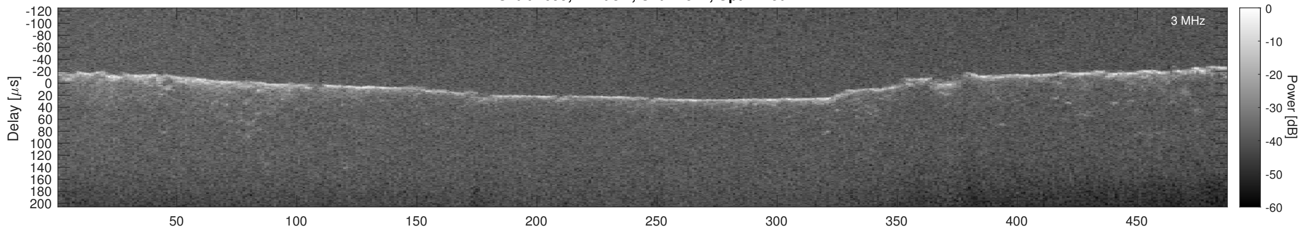
Orbit 4699, Cluttergram
