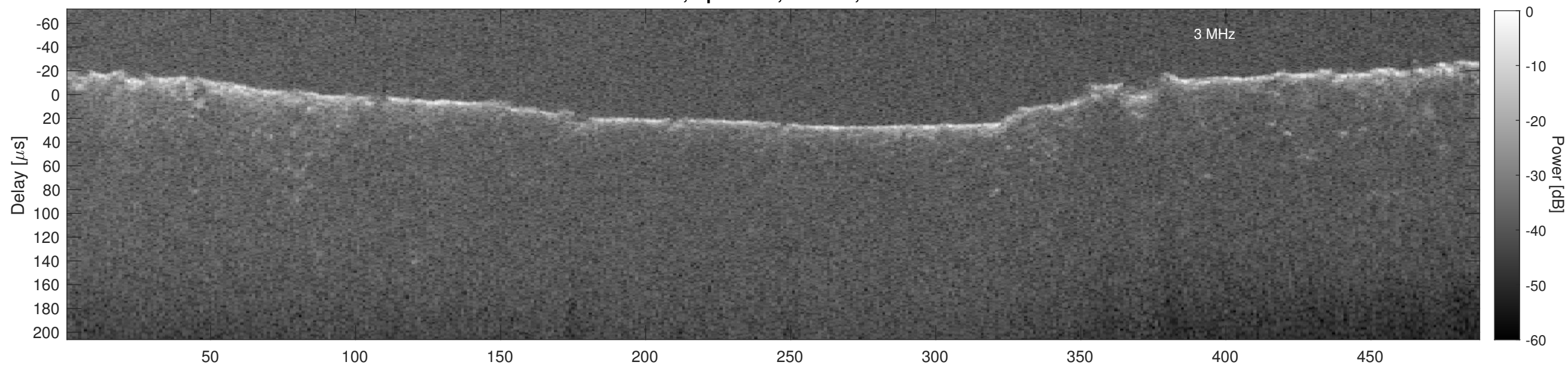
Orbit 4699, Cluttergram
