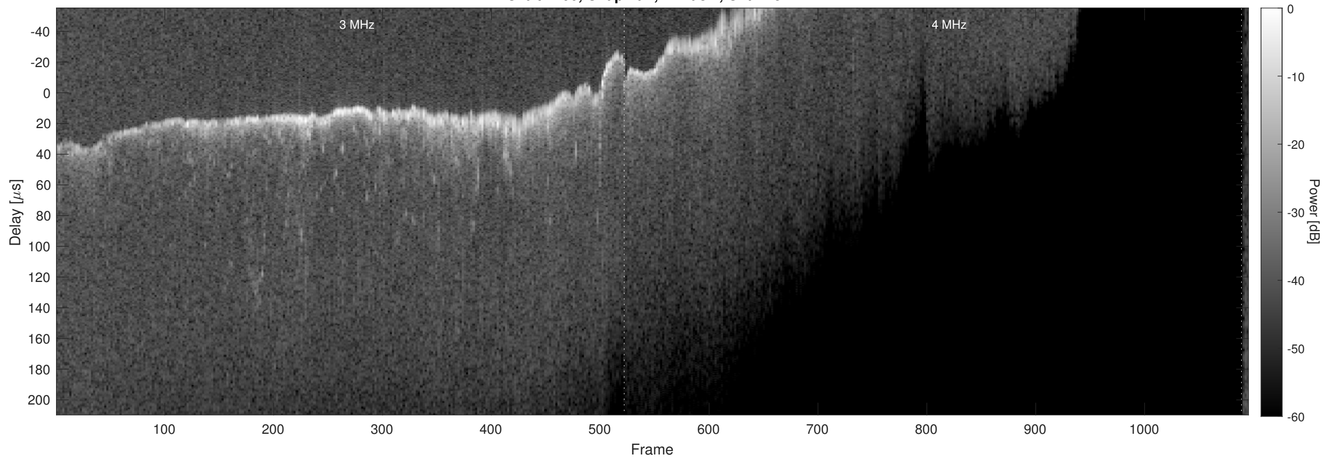
Orbit 4700, Chapman, Window, Channel 2
