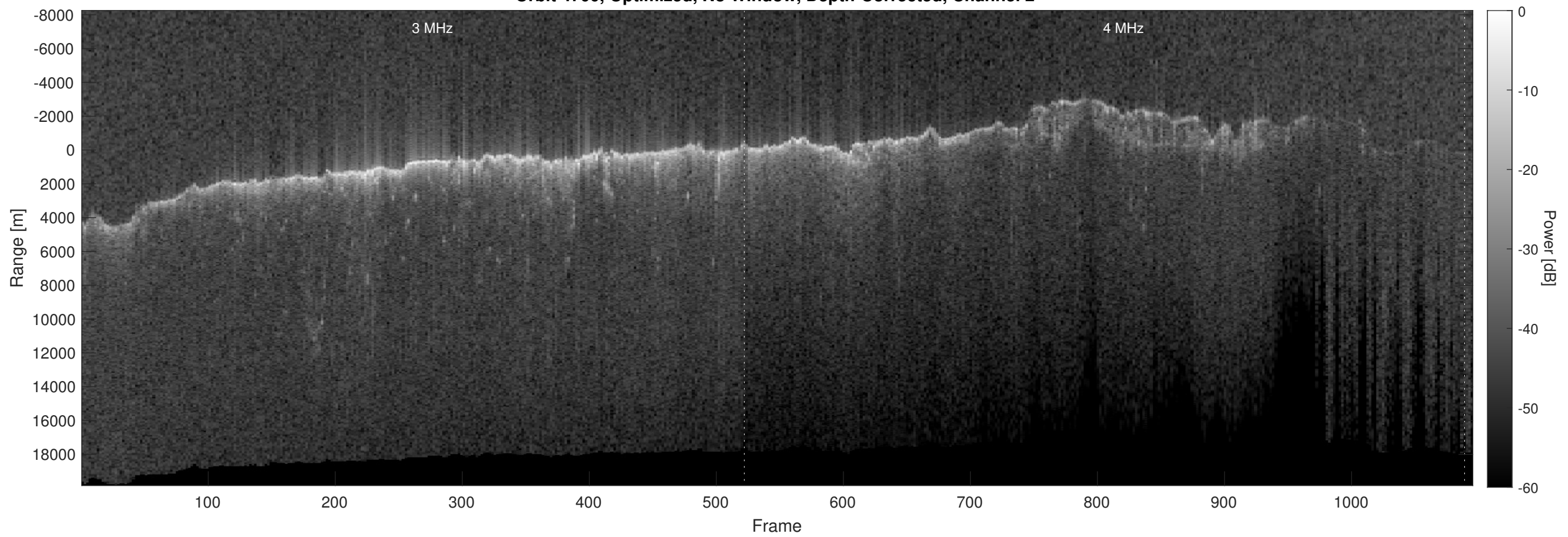
Orbit 4700, Optimized, No Window, Depth-Corrected, Channel 2
