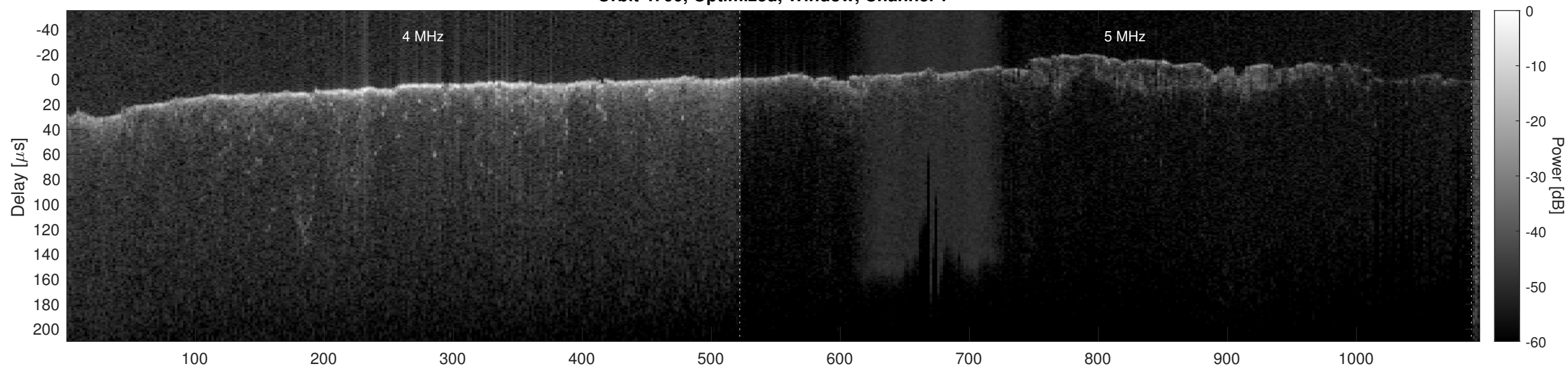
Orbit 4700, Optimized, Window, Channel 2
