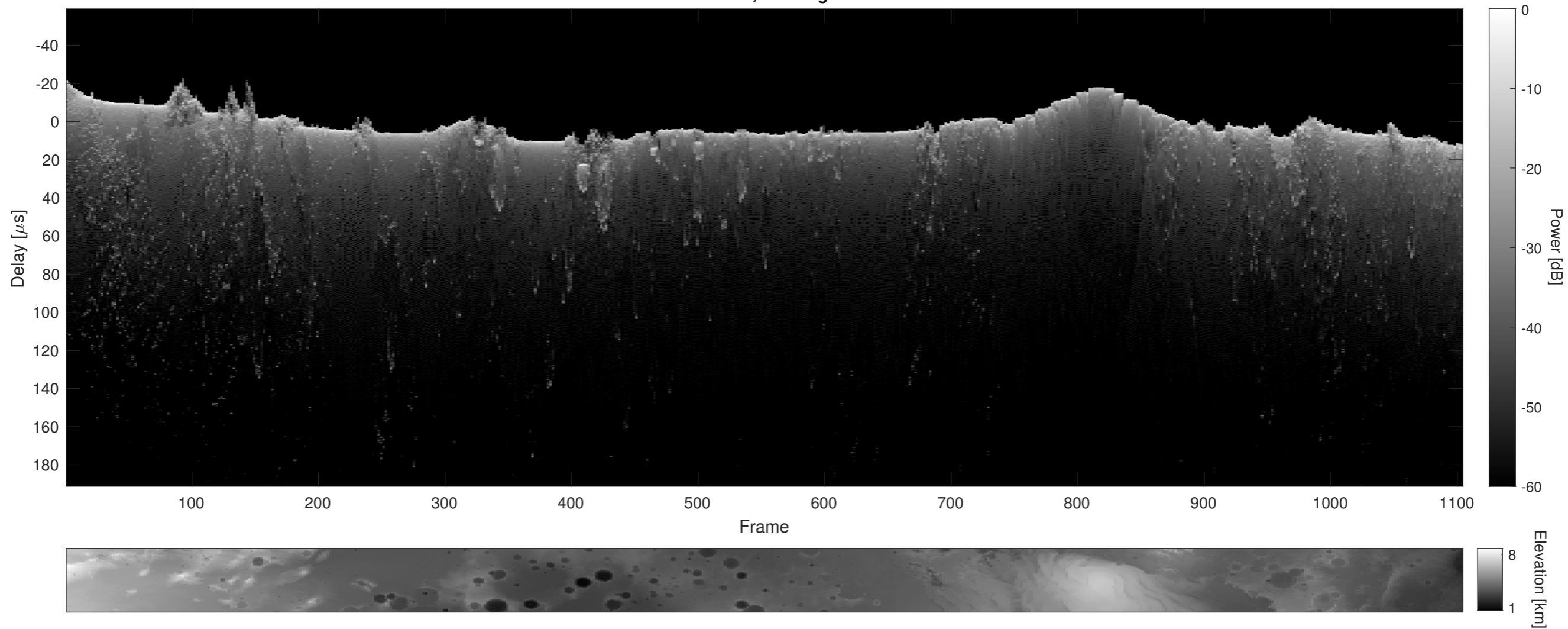
Orbit 4701, Cluttergram
