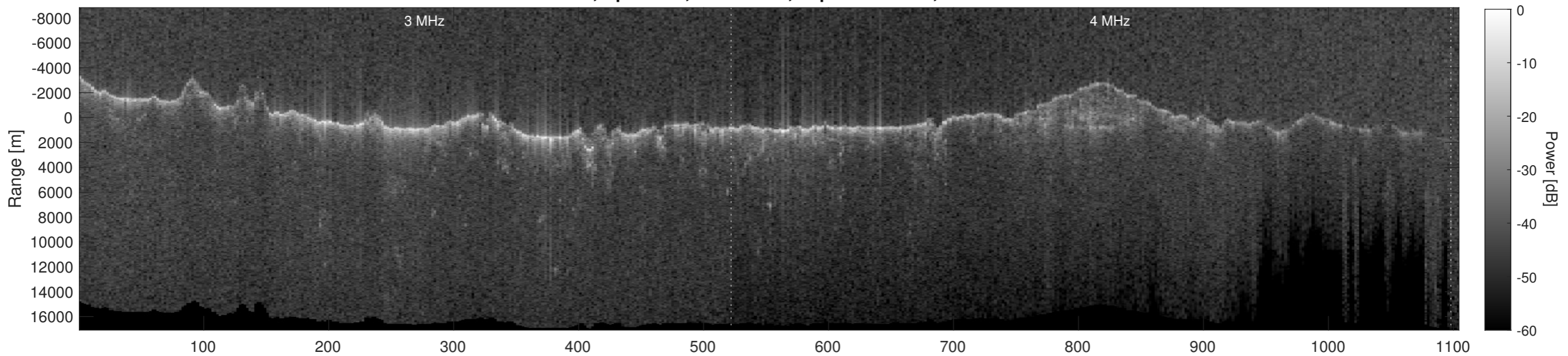
Orbit 4701, Depth-Corrected Cluttergram
