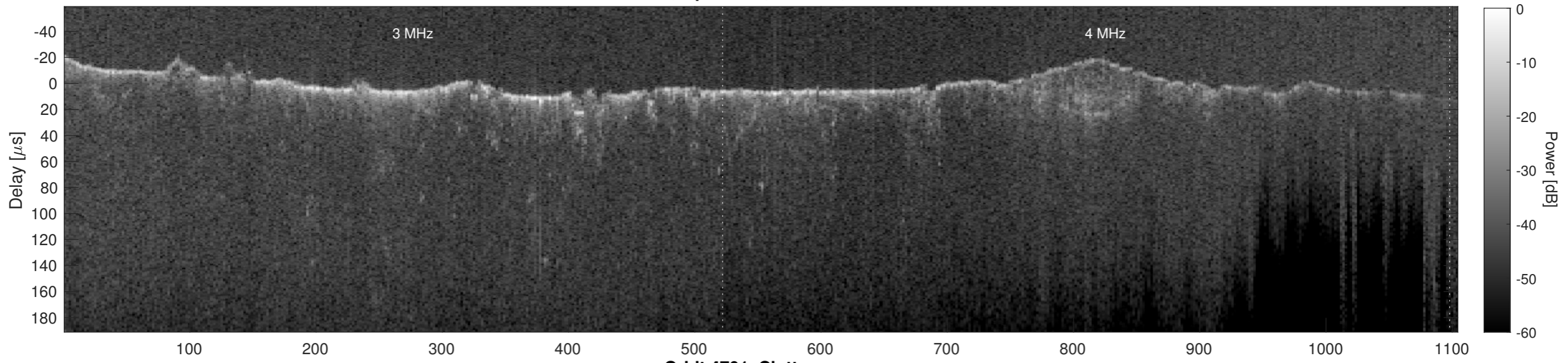
Orbit 4701, Cluttergram
