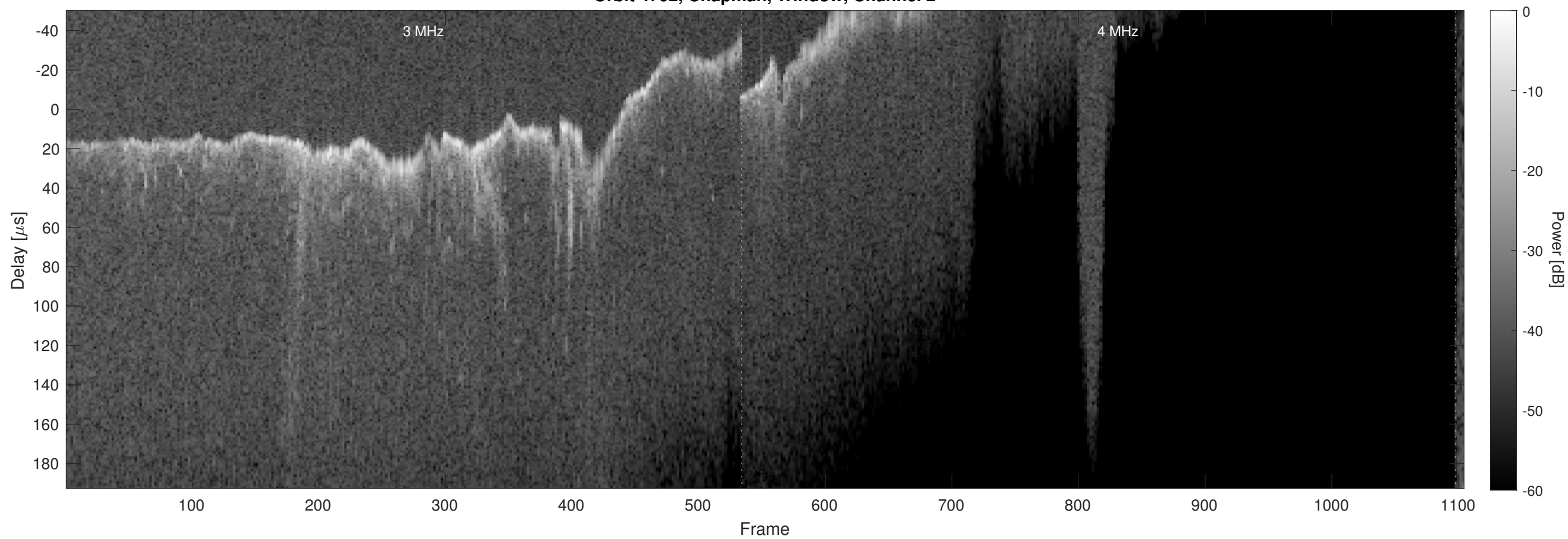
Orbit 4702, Chapman, Window, Channel 2
