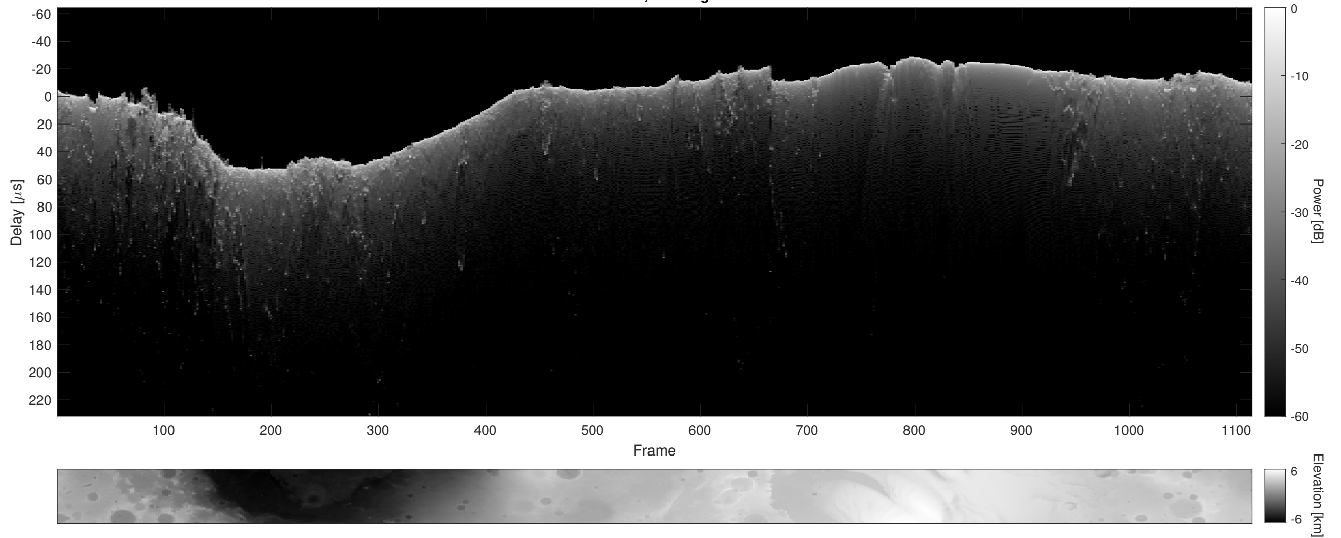
Orbit 4703, Cluttergram
