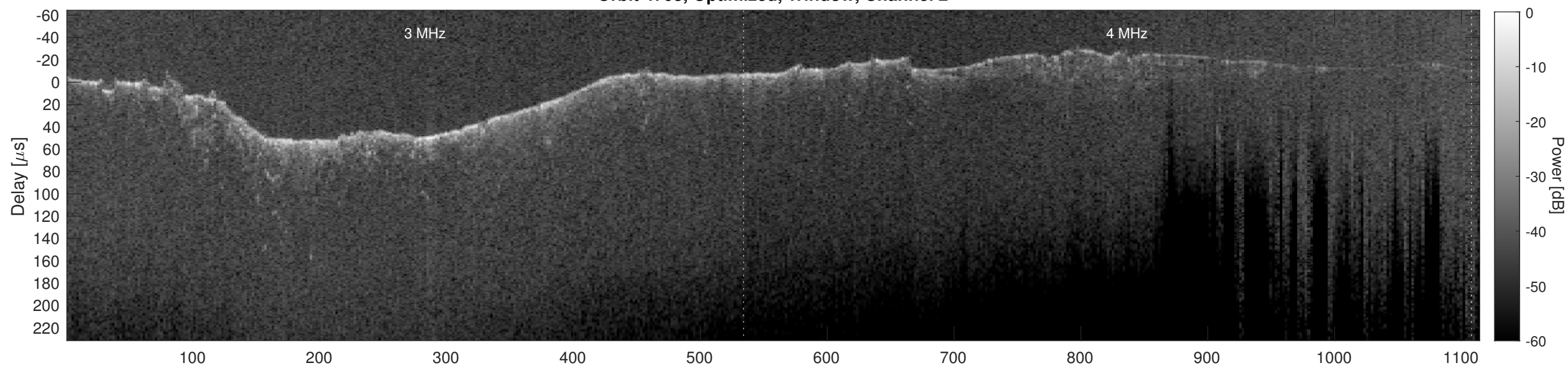
Orbit 4703, Cluttergram
