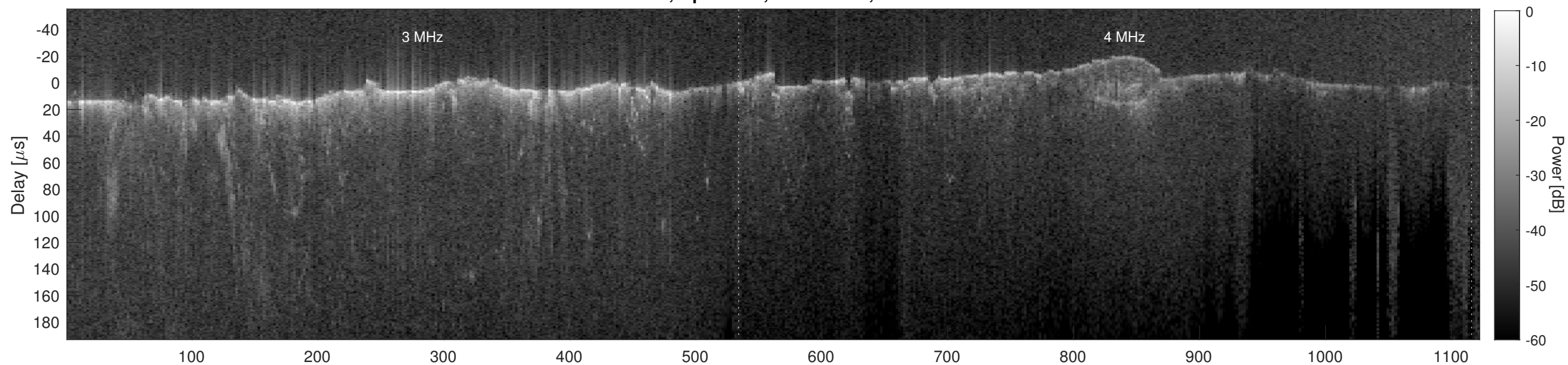
Orbit 4705, Cluttergram
