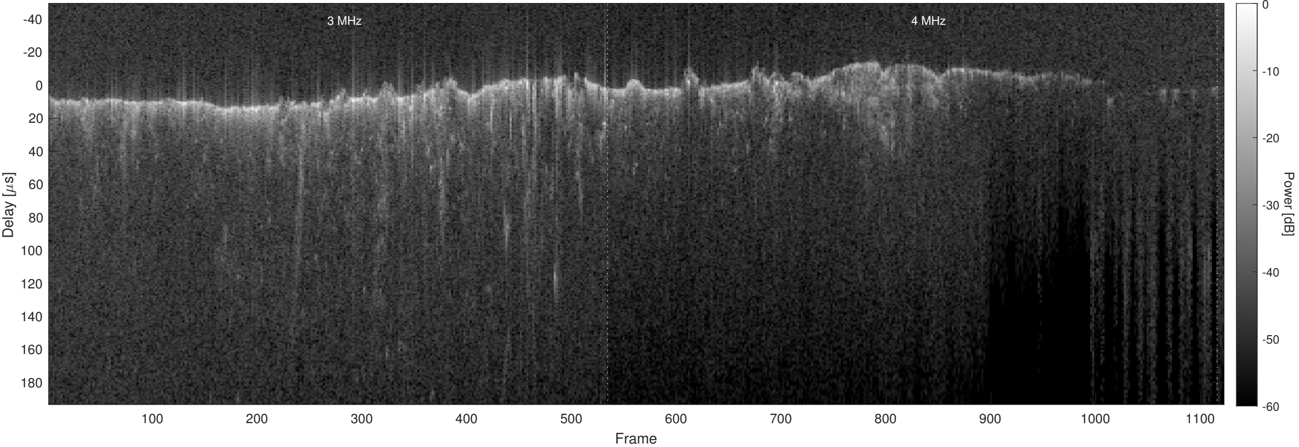
Orbit 4706, Optimized, No Window, Channel 2
