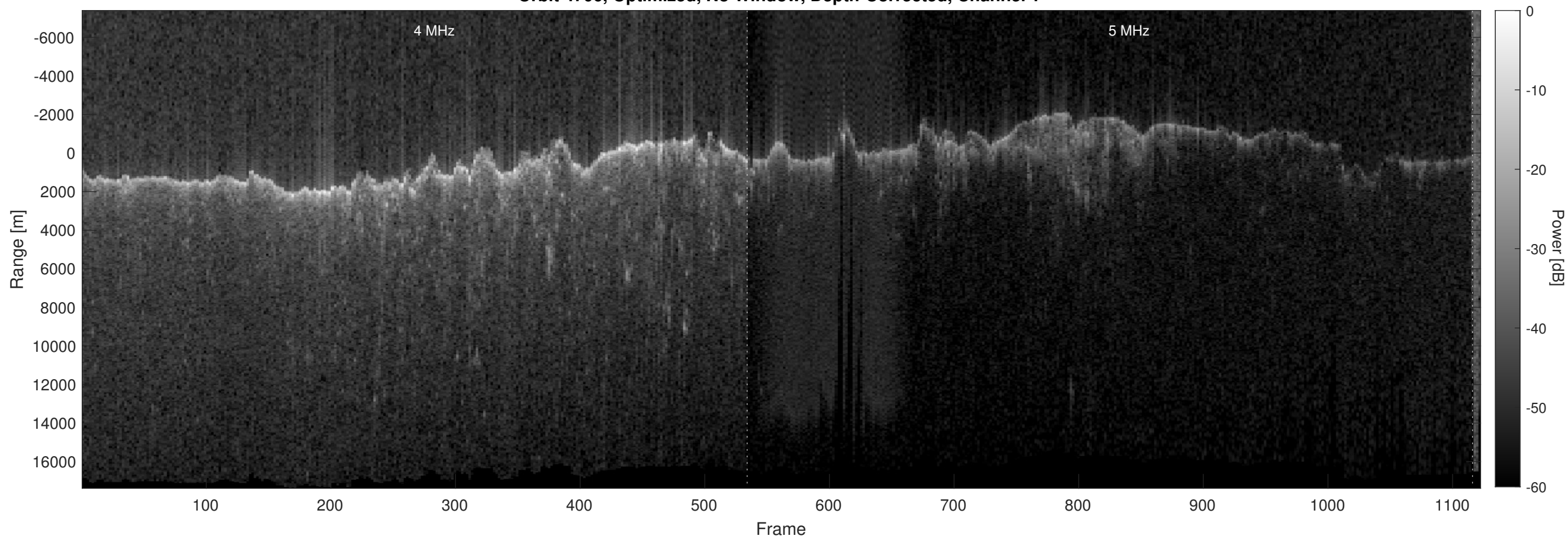
Orbit 4706, Optimized, No Window, Depth-Corrected, Channel 2
