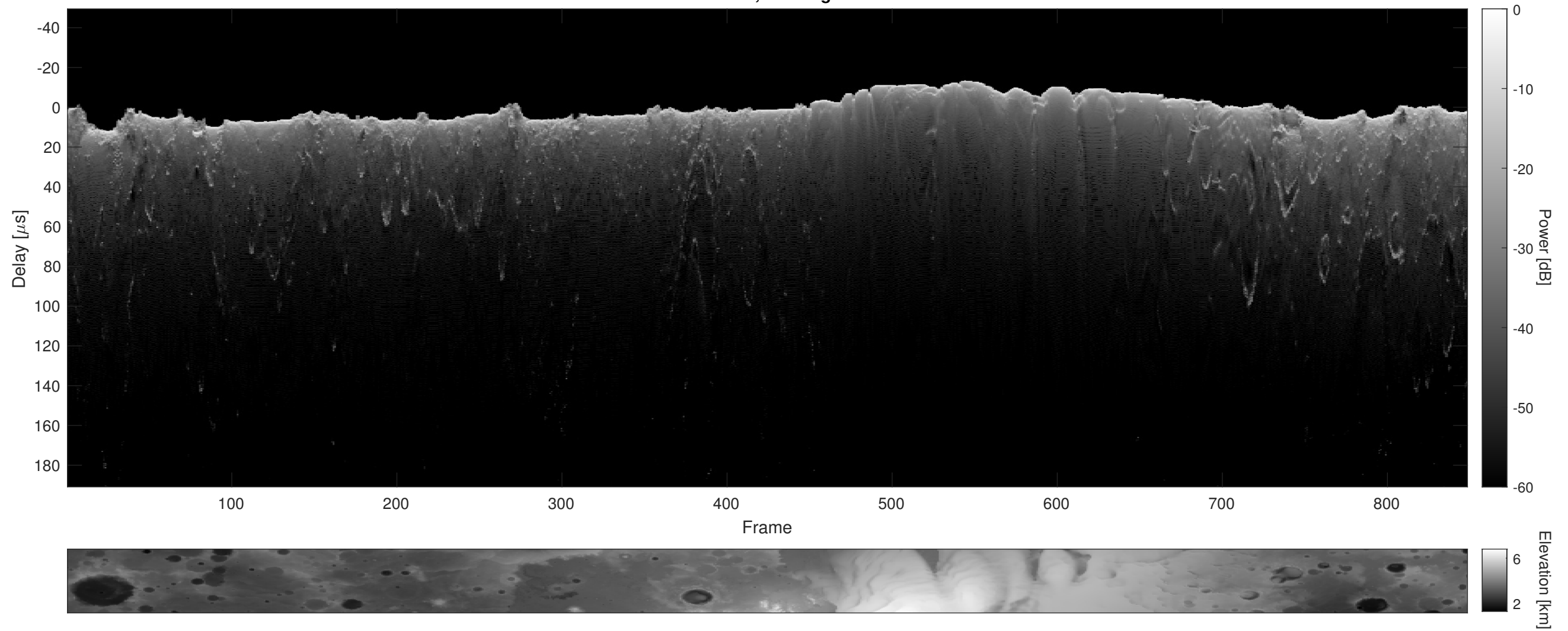
Orbit 4707, Cluttergram
