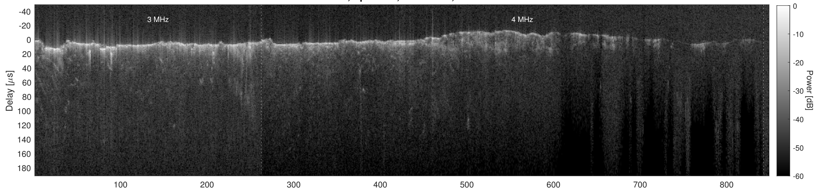
Orbit 4707, Cluttergram
