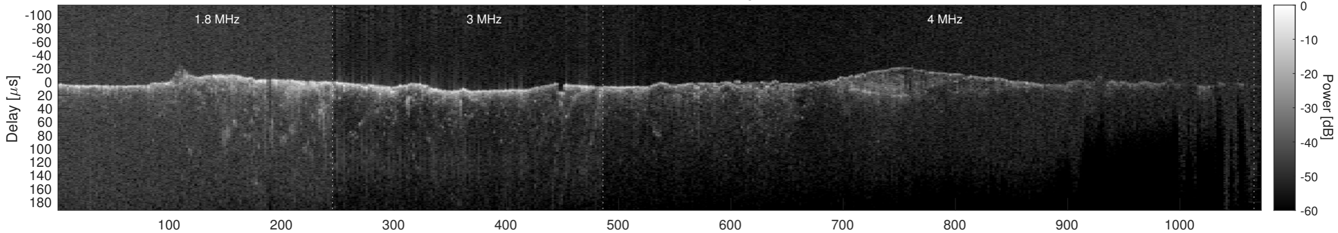
Orbit 4708, Cluttergram
