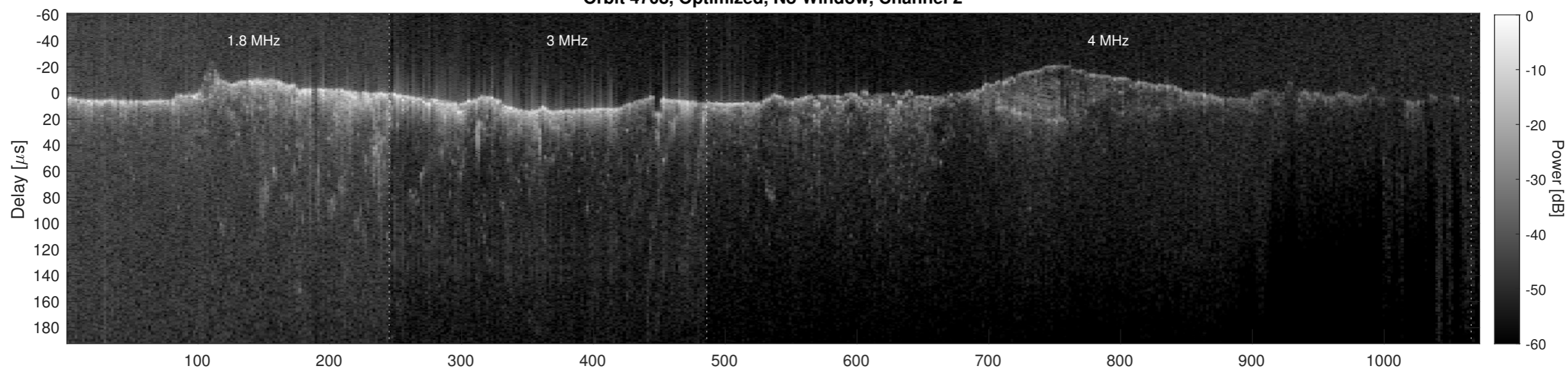
Orbit 4708, Cluttergram
