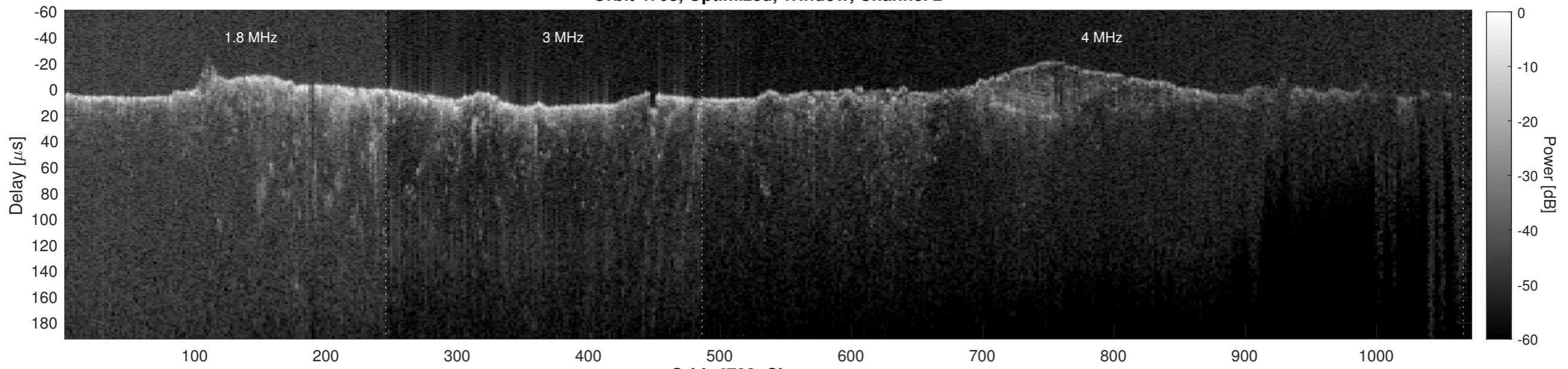
Orbit 4708, Cluttergram
