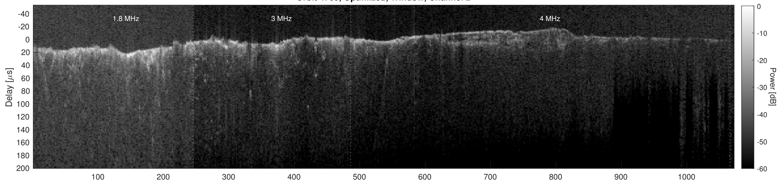
Orbit 4709, Cluttergram
