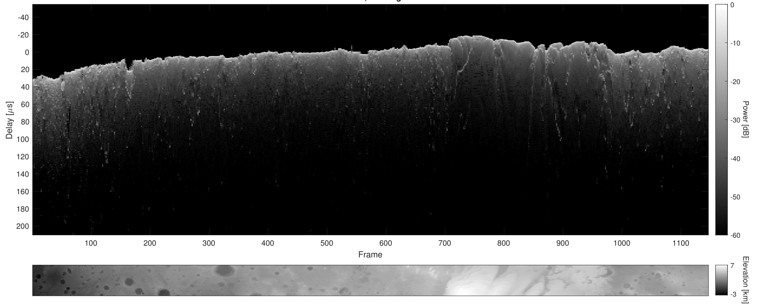
Orbit 4711, Cluttergram
