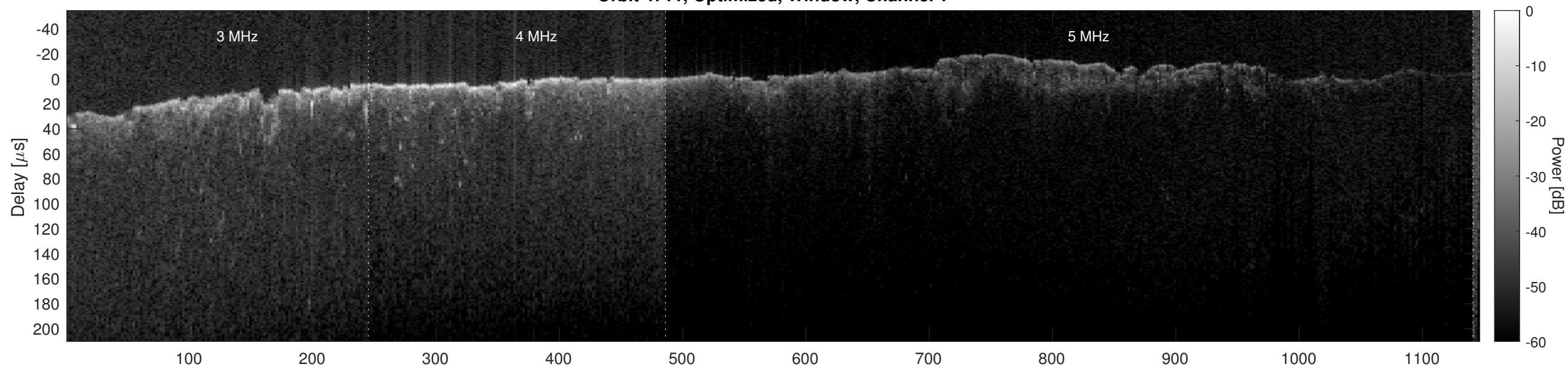
Orbit 4711, Optimized, Window, Channel 2
