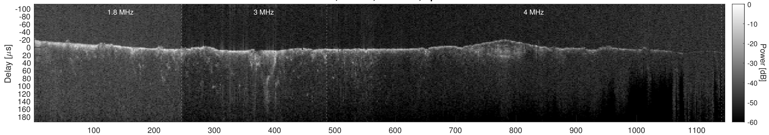
Orbit 4712, Cluttergram
