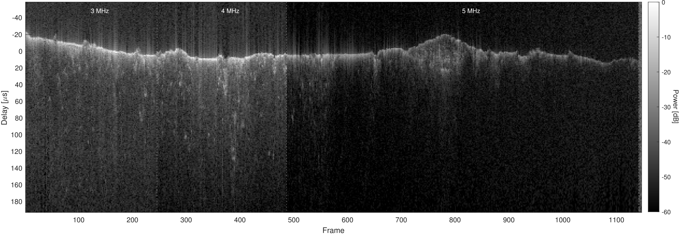
Orbit 4712, Optimized, No Window, Channel 2
