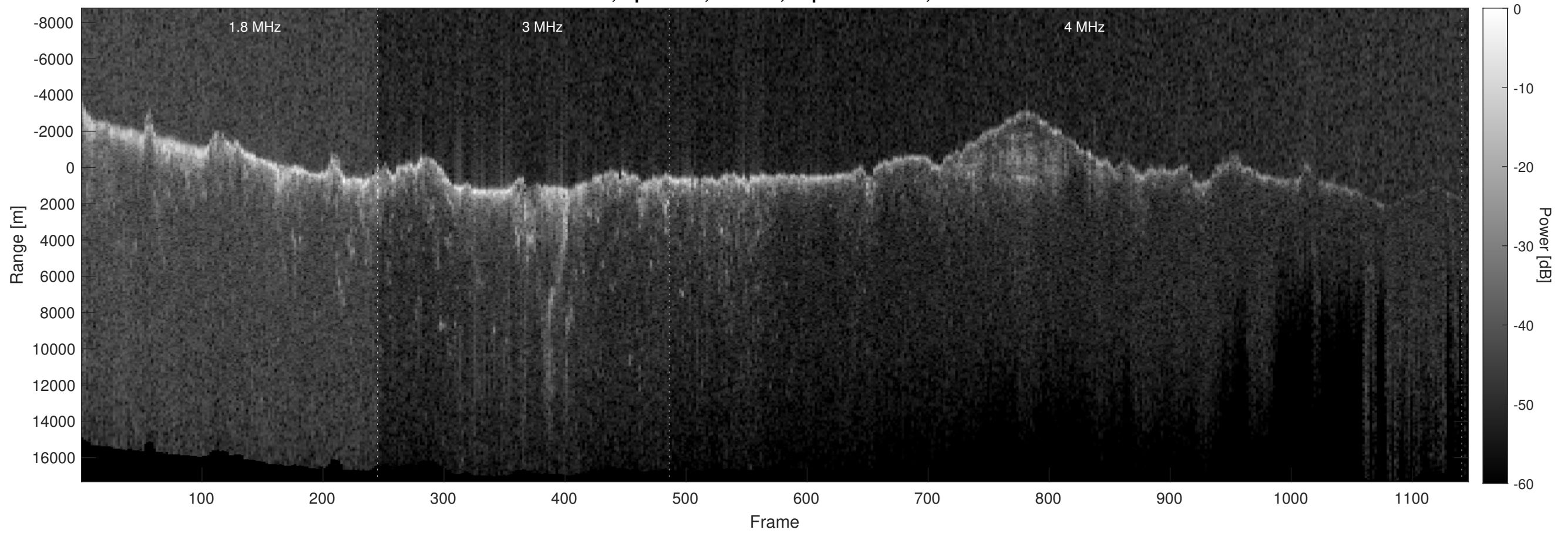
Orbit 4712, Optimized, Window, Depth-Corrected, Channel 2
