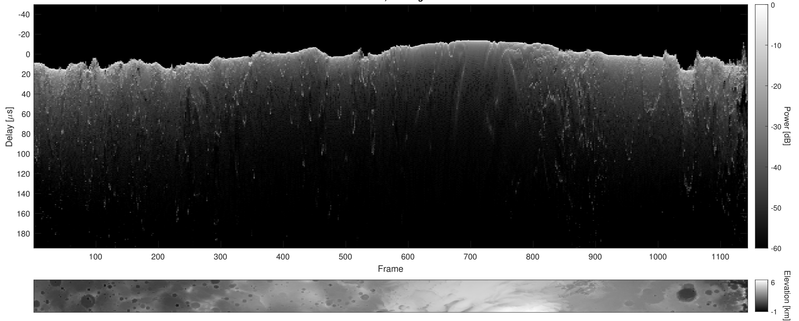
Orbit 4713, Cluttergram
