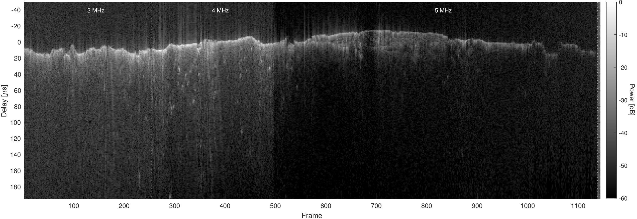
Orbit 4713, Optimized, No Window, Channel 2
