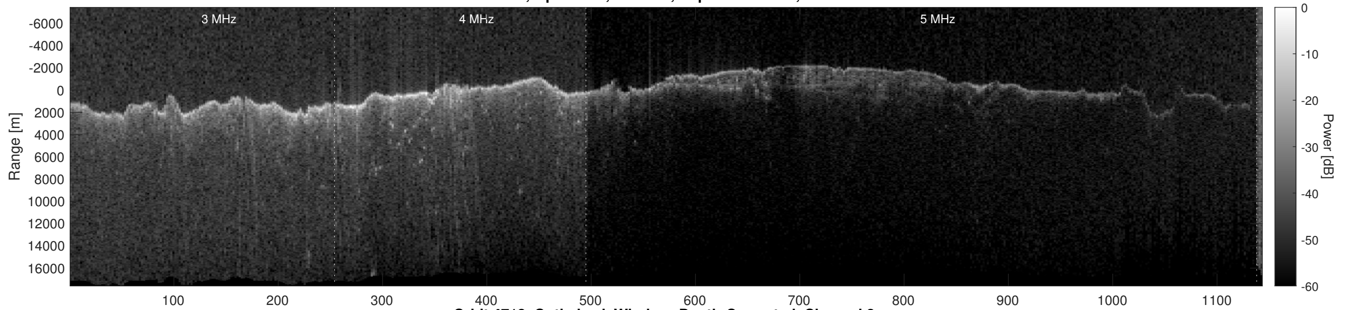
Orbit 4713, Optimized, Window, Depth-Corrected, Channel 2
