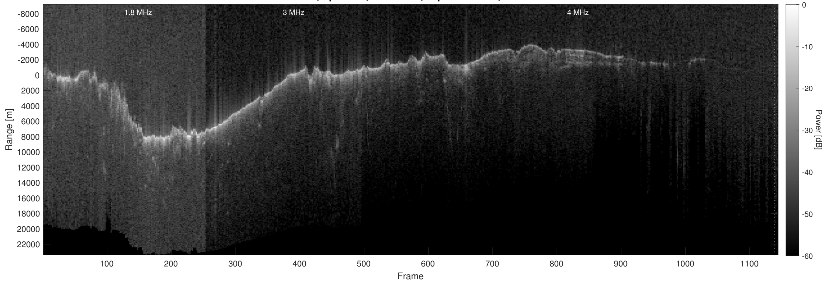
Orbit 4714, Optimized, No Window, Depth-Corrected, Channel 2
