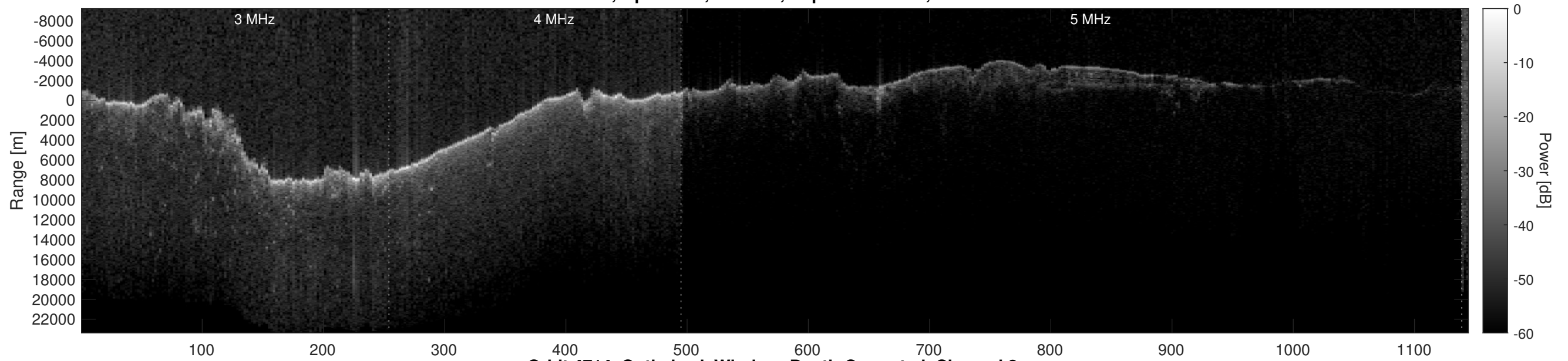
Orbit 4714, Optimized, Window, Depth-Corrected, Channel 2
