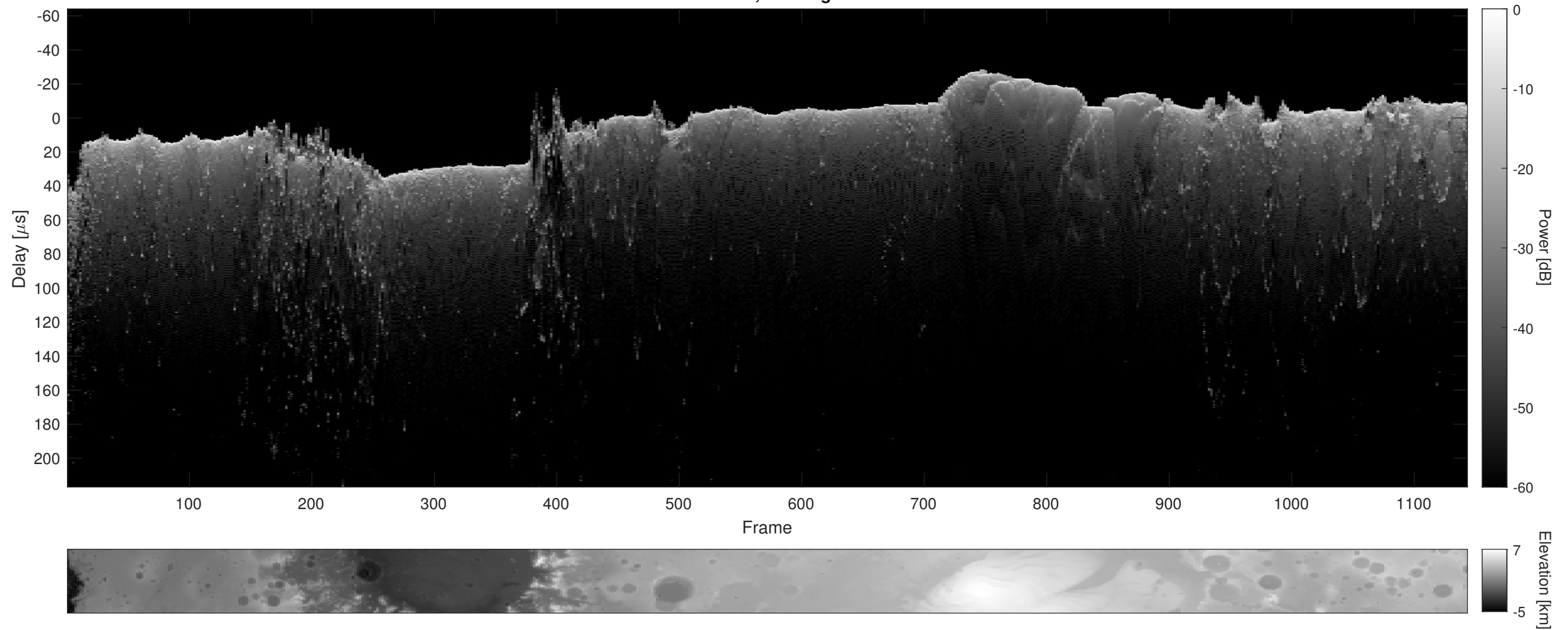
Orbit 4715, Cluttergram
