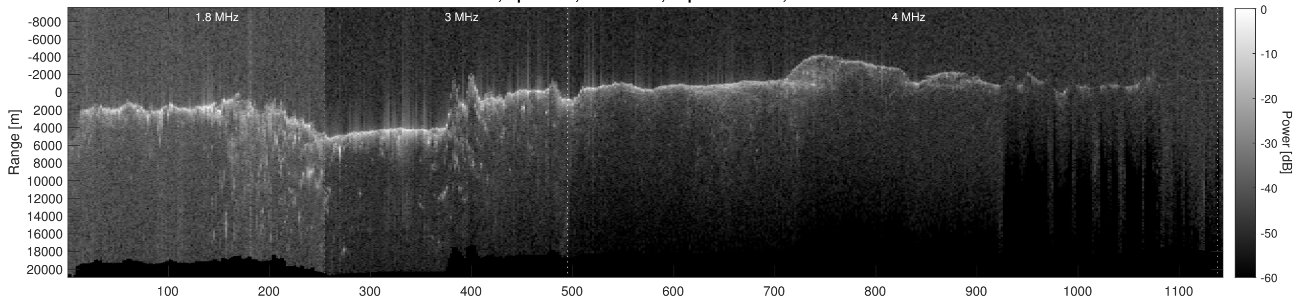
Orbit 4715, Depth-Corrected Cluttergram
