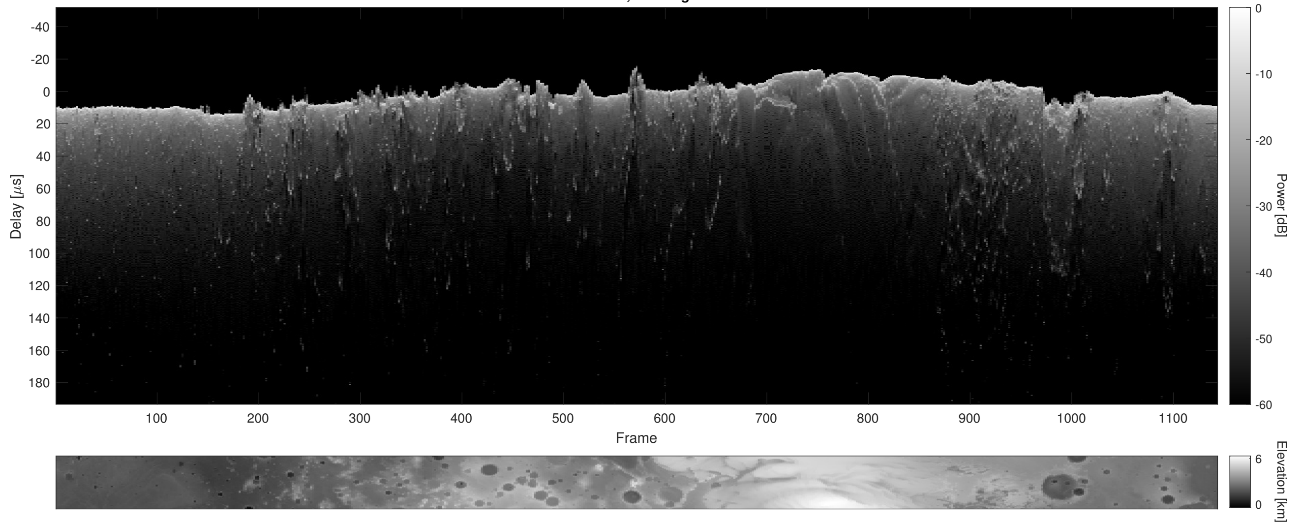
Orbit 4717, Cluttergram
