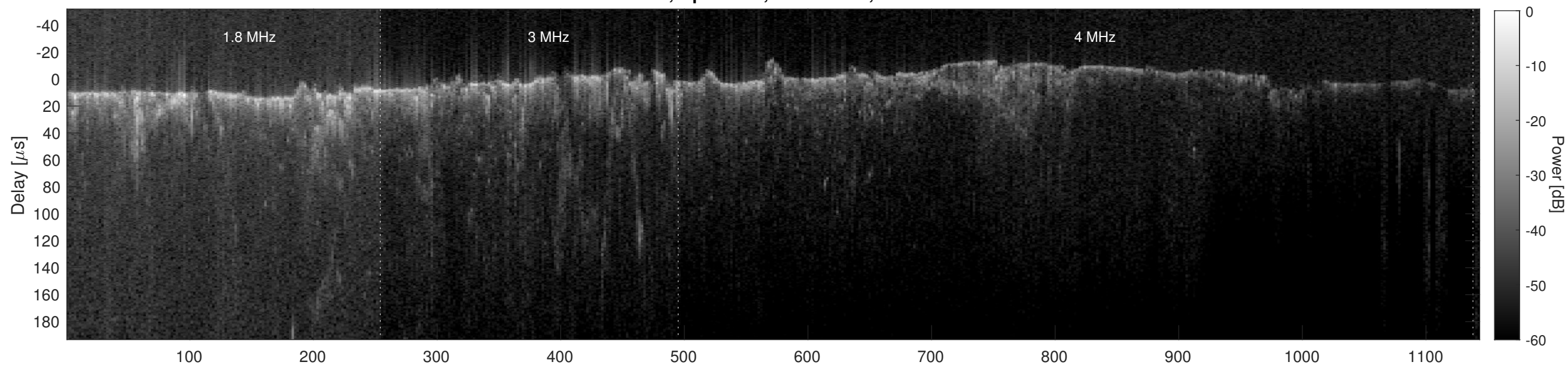
Orbit 4717, Cluttergram
