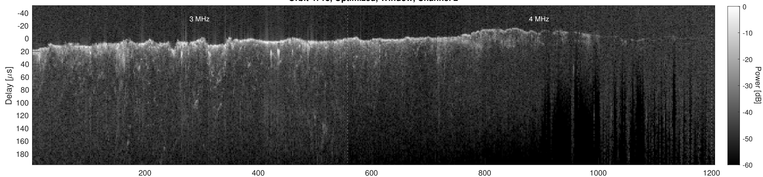
Orbit 4718, Cluttergram
