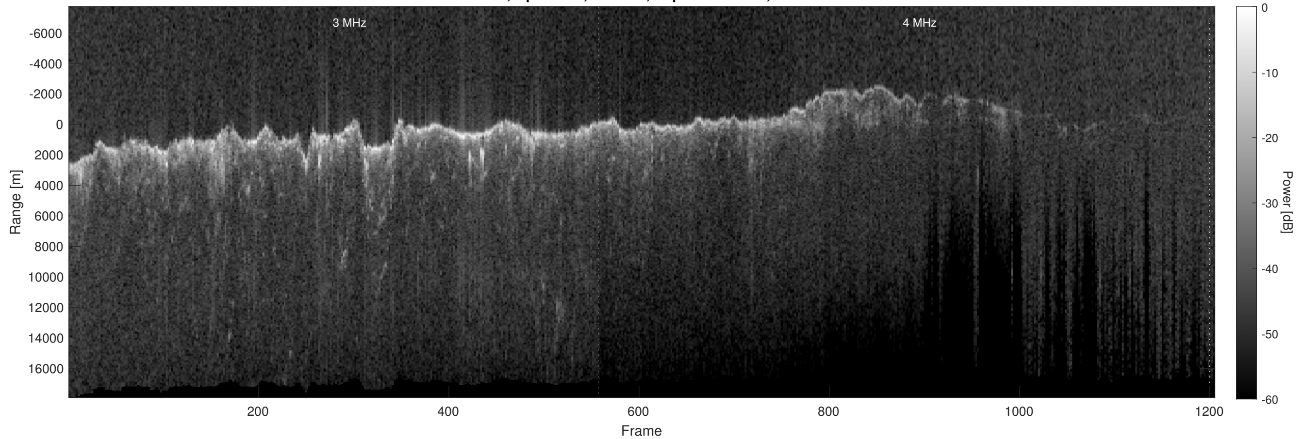
Orbit 4718, Optimized, Window, Depth-Corrected, Channel 2
