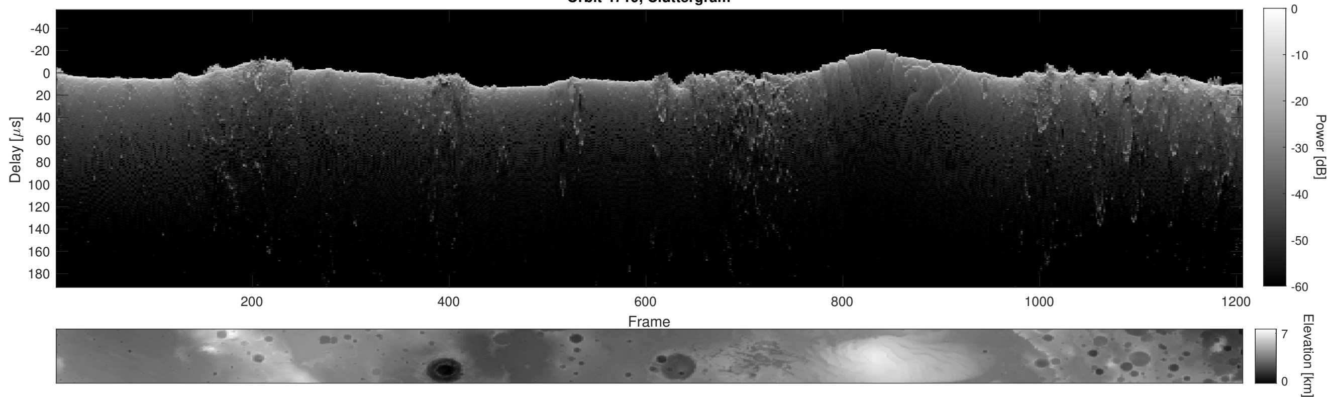
Orbit 4719, Cluttergram
