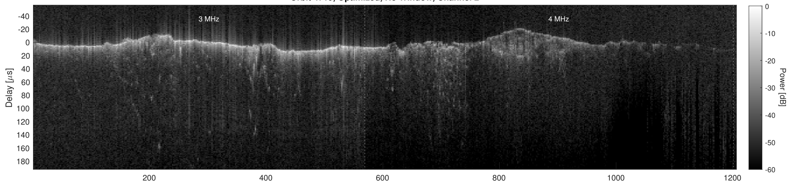
Orbit 4719, Cluttergram
