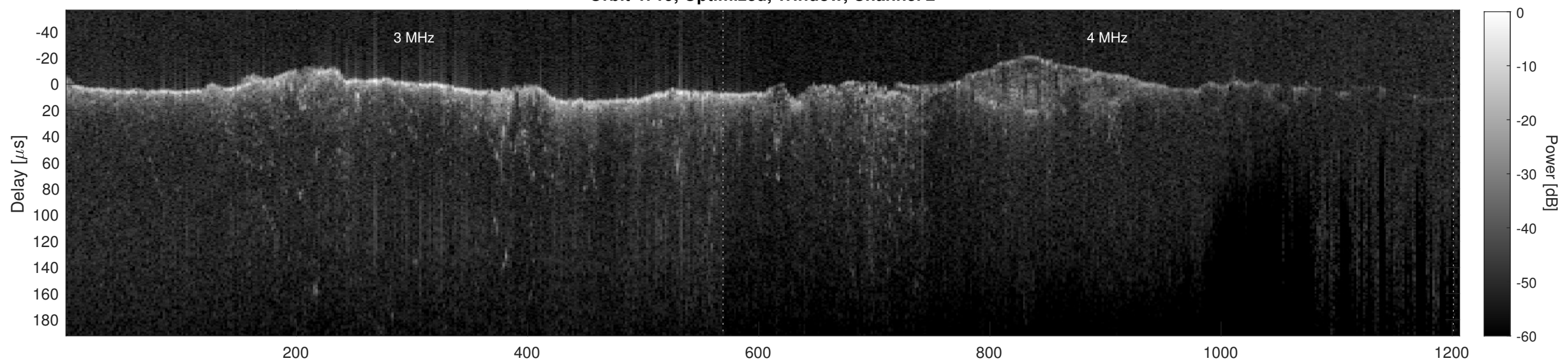
Orbit 4719, Cluttergram
