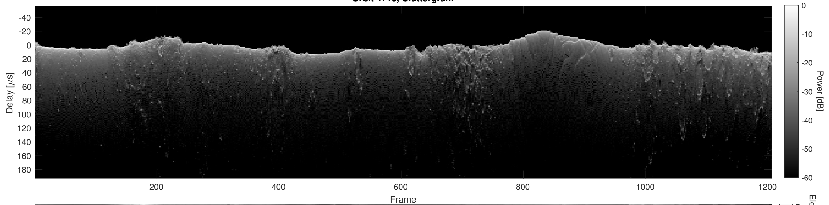
Orbit 4719, Cluttergram
