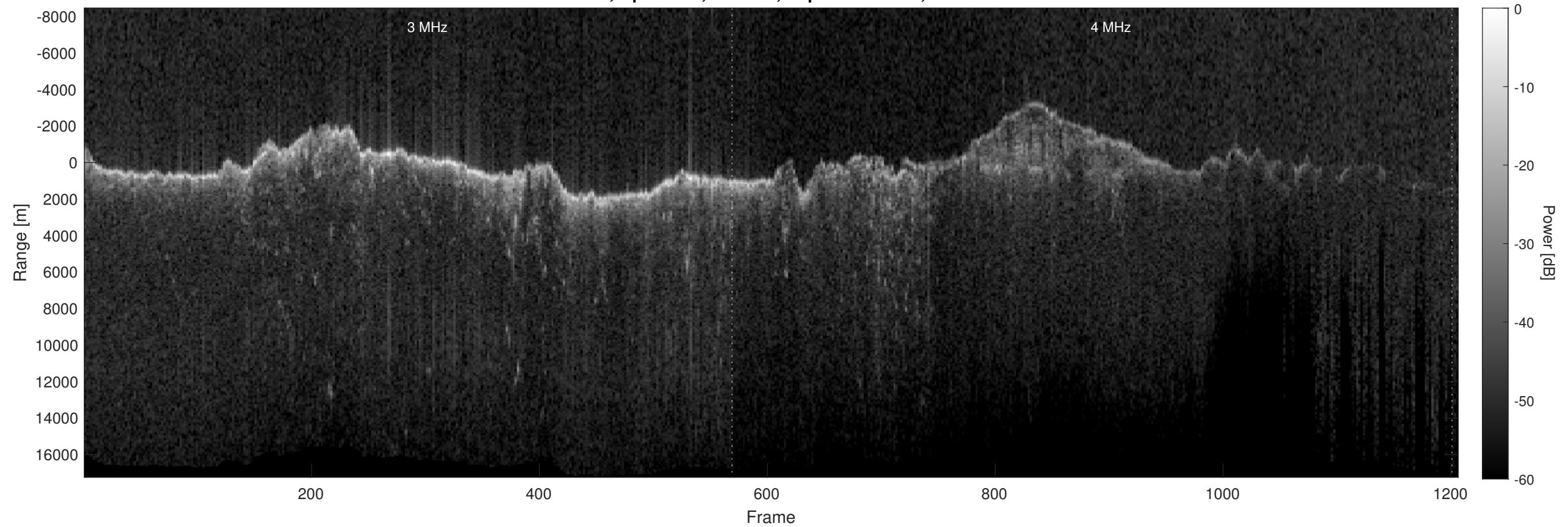
Orbit 4719, Optimized, Window, Depth-Corrected, Channel 2
