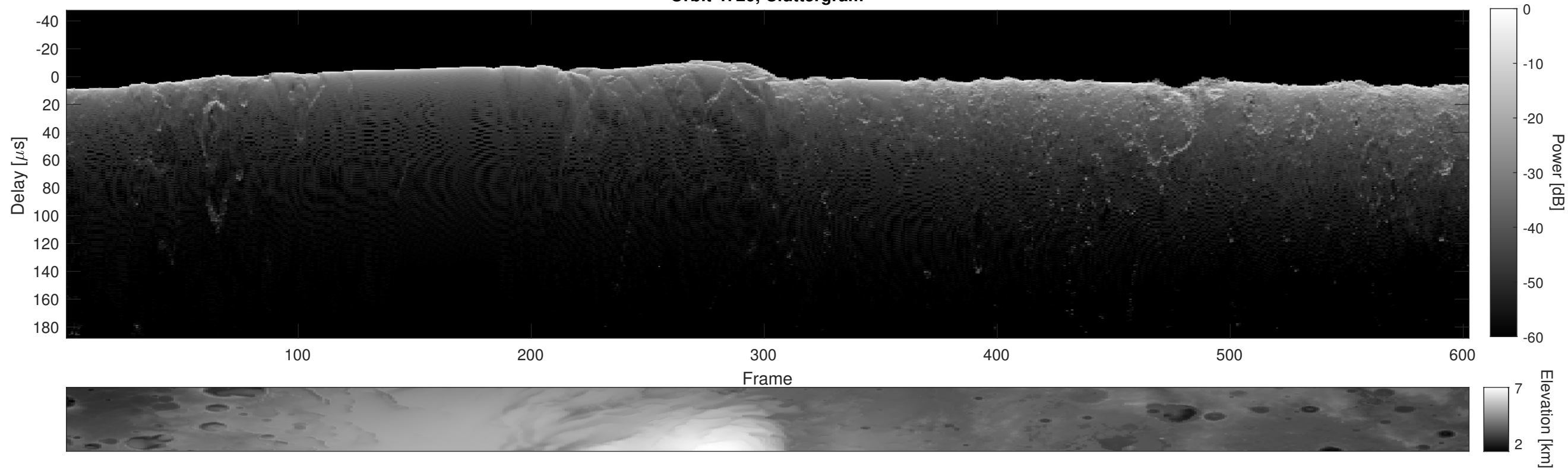
Orbit 4720, Cluttergram
