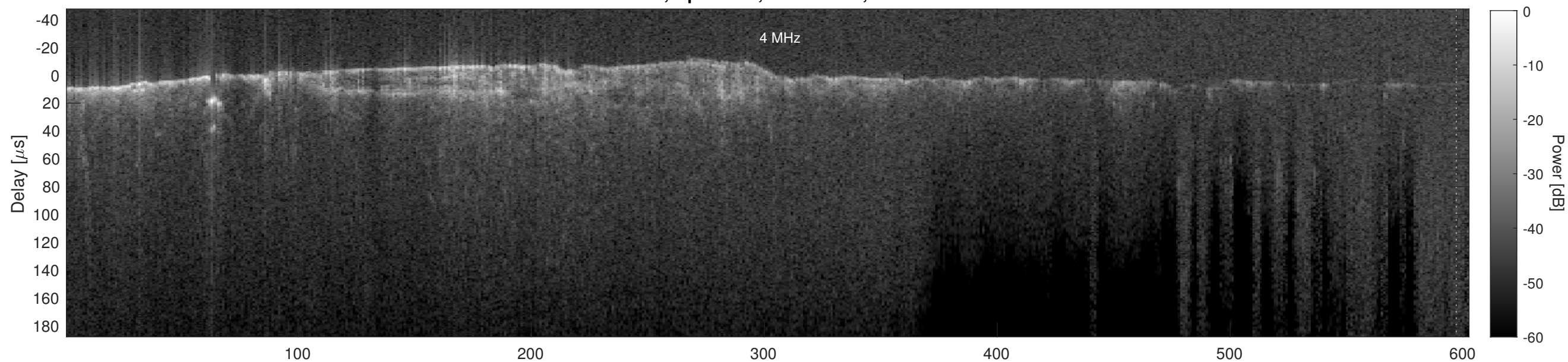
Orbit 4720, Cluttergram
