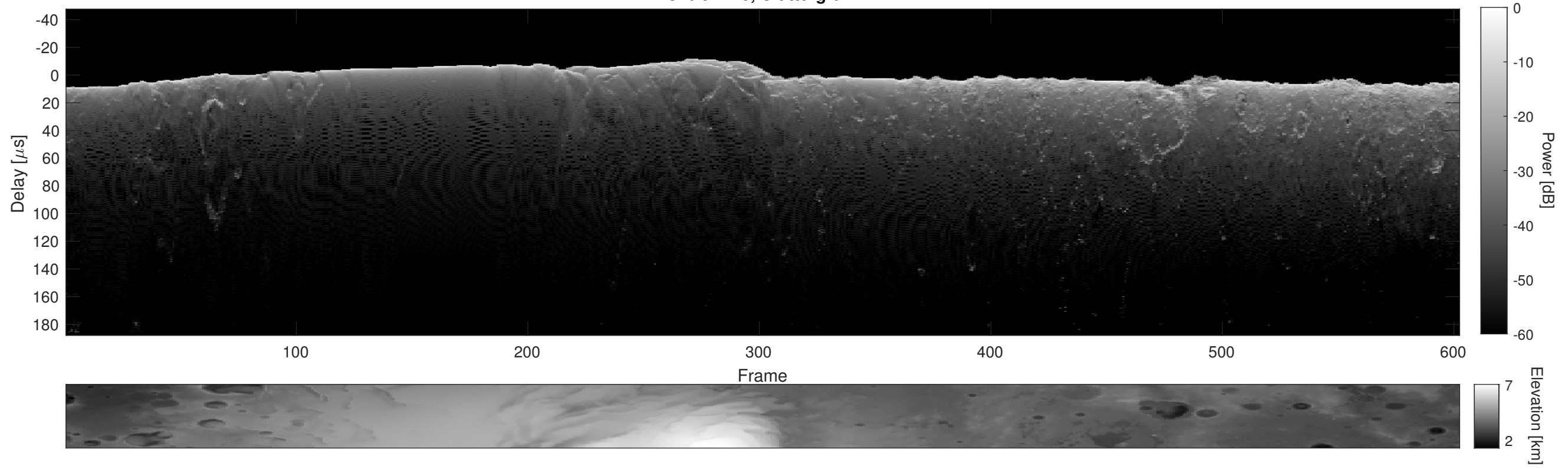
Orbit 4720, Cluttergram
