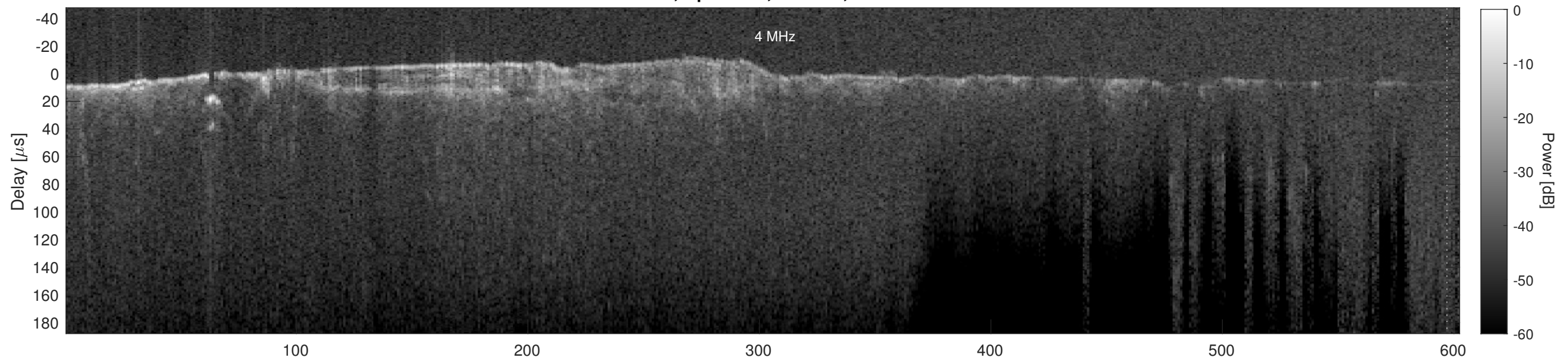
Orbit 4720, Cluttergram
