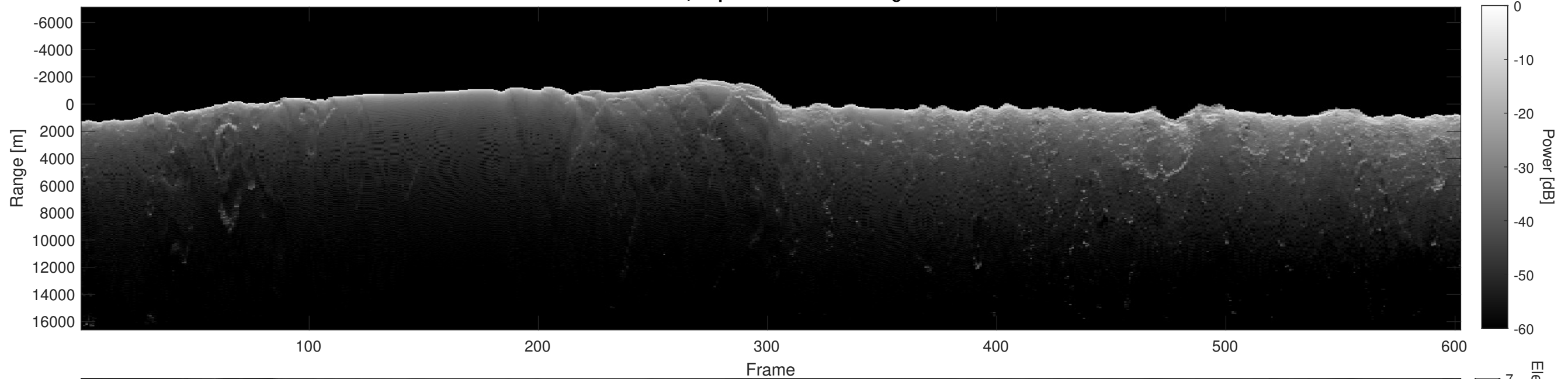
Orbit 4720, Depth-Corrected Cluttergram
