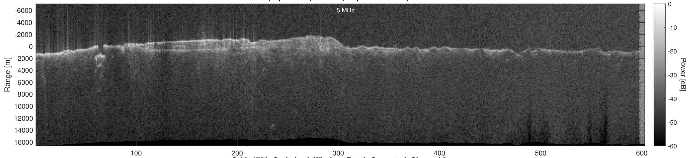
Orbit 4720, Optimized, Window, Depth-Corrected, Channel 2
