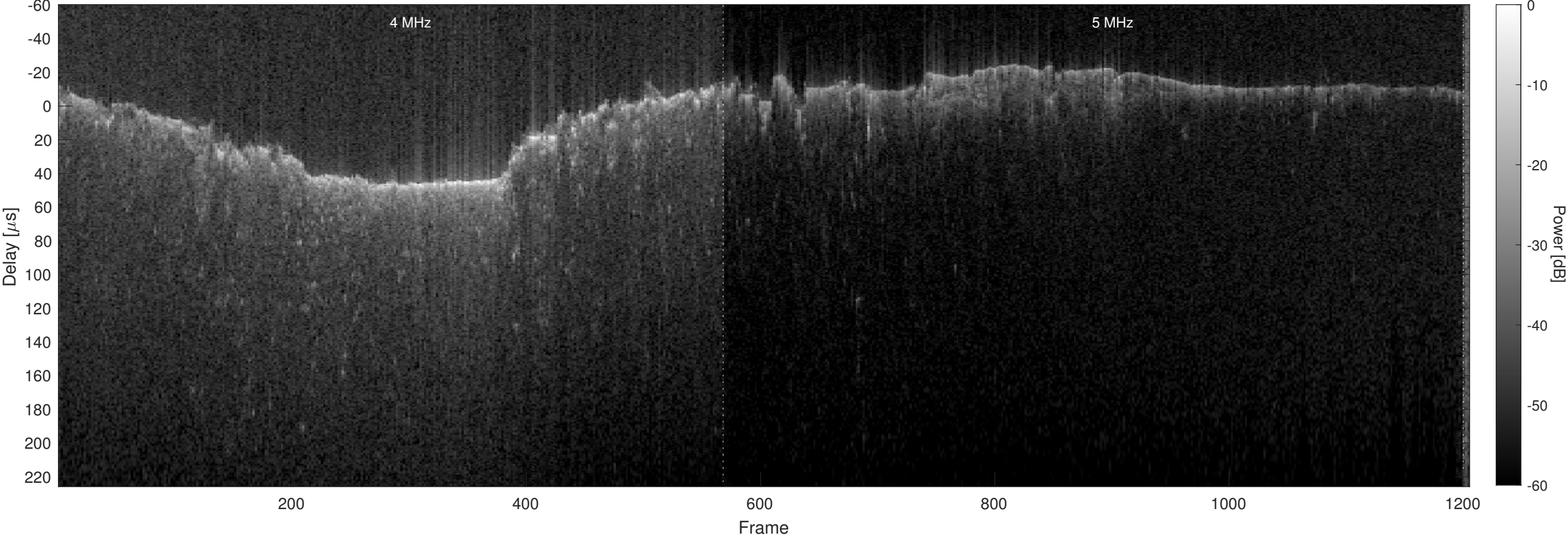
Orbit 4721, Optimized, No Window, Channel 2
