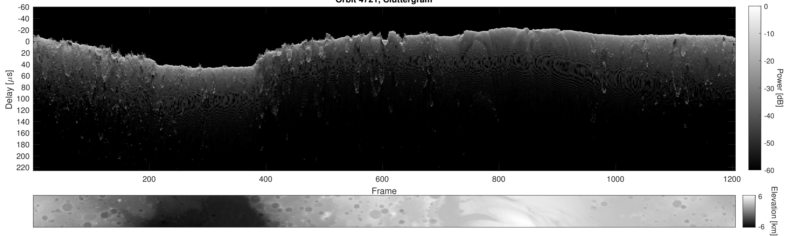
Orbit 4721, Cluttergram
