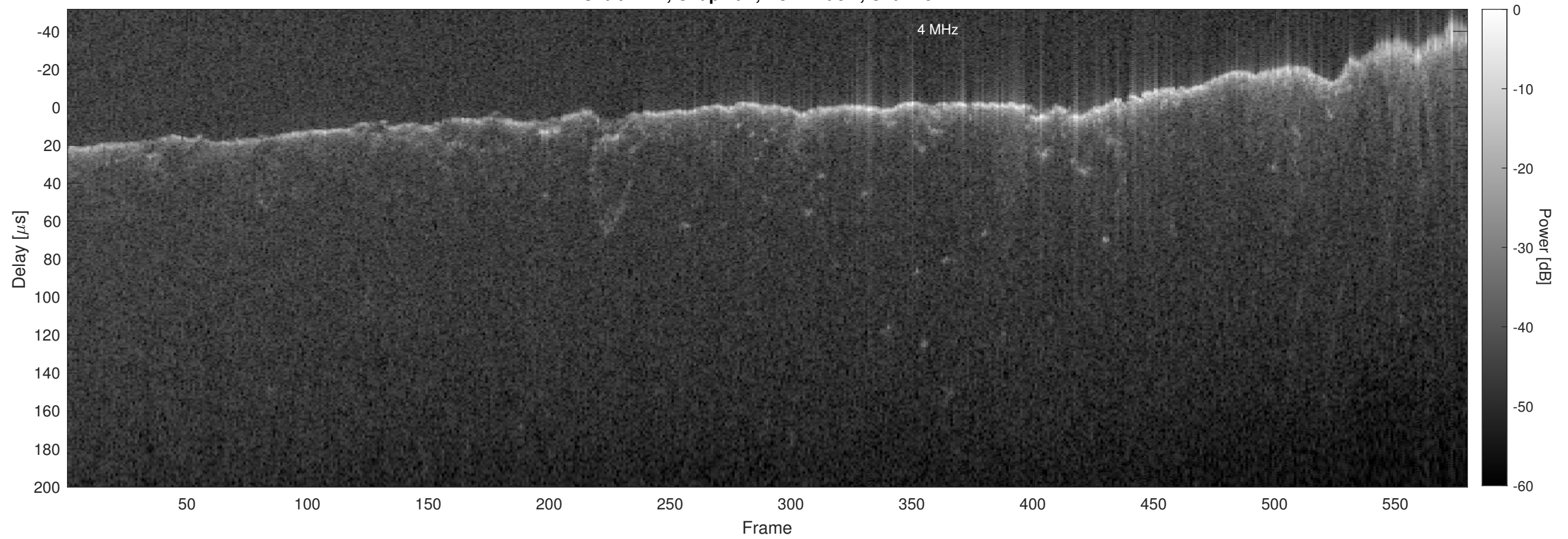
Orbit 4722, Chapman, No Window, Channel 2
