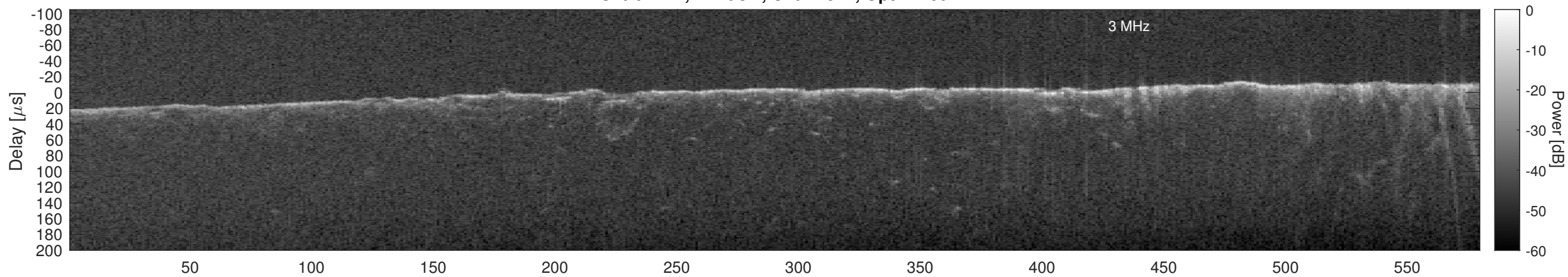
Orbit 4722, Cluttergram
